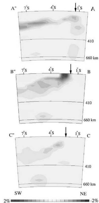
Figure 3. Cross-sections (at true scale) showing high-velocity zone beneath New Guinea. Refer to Figure 1 for the geographical locations of the sections. Arrows indicate the location of the coastline in each cross-section. See color version of this figure in the HTML.
