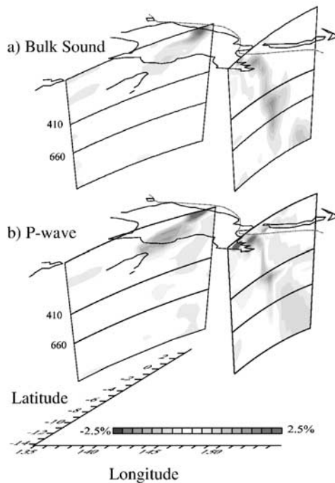
Figure 2. Cross-sections of the bulk-sound tomographic model and P-wave model, showing southwestward subduction at the New Guinea Trench (left) and northward subduction at the New Britain Trench (right). See color version of this figure in the HTML.
