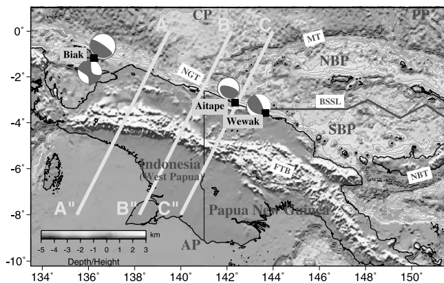
Figure 1. Configuration of tectonic boundaries in Papua New Guinea and eastern Indonesia. Available CMT focal mechanisms ( M_w > 7 ) are plotted for events located reliably on the New Guinea Trench (plus the 1979 Yapen strike-slip event). Lines in yellow indicate surface traces of tomographic cross-sections (see Figure 3). AP: Australian Plate; BSSL: Bismarck Sea Seismic Lineation; CP: Caroline Plate; FTB: Highlands Fold-and-Thrust Belt; MT: Manus Trench; NBP: North Bismarck Plate; NBT: New Britain Trench; NGT: New Guinea Trench; SBP: South Bismarck Plate; PP: Pacific Plate. See color version of this figure in the HTML.
