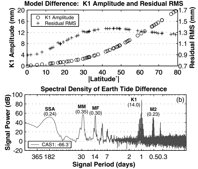
Figure 1. a) K1 amplitude and residual RMS of the solid Earth tide model differences (IERS 2003 - IERS 1992), in the vertical component as a function of the absolute value of site latitude. b) PSD of the vertical component of the model differences at the CAS1 site (note the signal amplitudes in mm within brackets).
