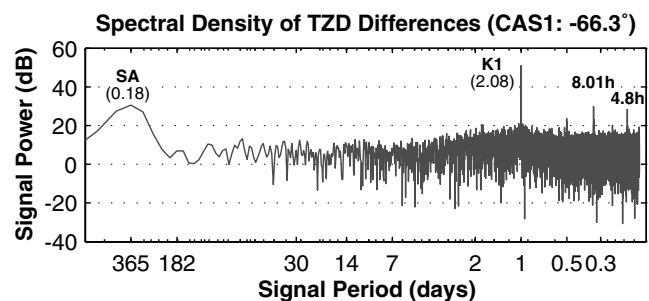
Figure 5. Power spectral density of the ZTD differences at the CAS1 site.
