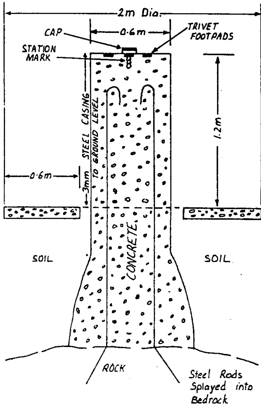
CROSS SECTION SURVEY STATION PILLAR Photo Identification:
