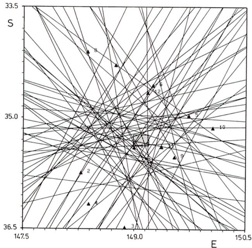
Figure 3. Practical example of the arrival order method for an event near station CAN in Fig. 5, illustrating the 66 constraints imposed by time picks at 12 stations. The rectangular zone needed for further inversion is stippled.
