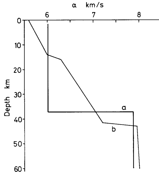
Figure 6. Velocity models for the crustal structure in SE Australia: (a) the simple regional model of Doyle, Everingham & Hogan (1959), (b) averaged velocity model for the Dalton/Gunning zone derived from the work of Finlayson & McCracken (1981).
