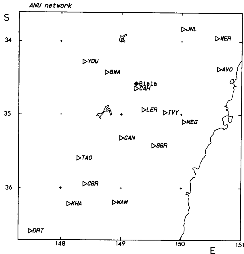
Figure 5. The SE Australian seismic network administered by the Australian National University, with the location of the earthquake at Biala illustrated in Figs 7 and 8.
