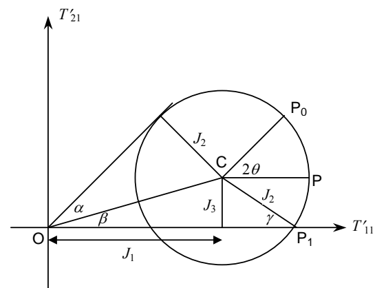
Figure 1. Mohr circle representation of the phase tensor.
