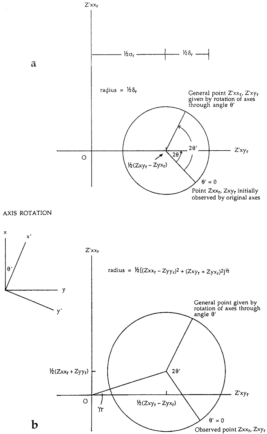
Fig. 1. Mohr circles for the values taken by the elements of a magnetotelluric impedance tensor, upon rotation of the measuring axes through angle \theta' . a. Circle for a 2-D structure; b. Circle for a 3-D structure. For a 1-D structure, the circle in Fig. 1a reduces to its central point. Similar diagrams can be drawn for the quadrature elements.
